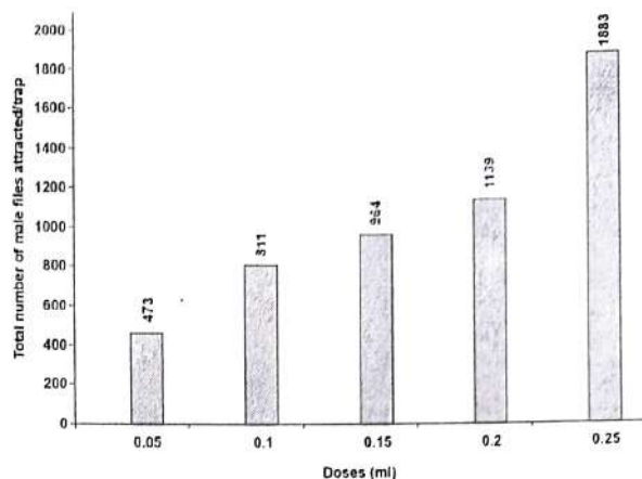
Fig. 1. Effect of doses of Cure-lure on attraction of males of B. cucurbitae
